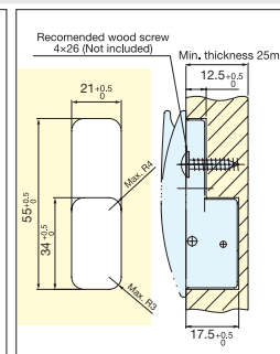
Bore Dimensions (For thickness 25~29 mm)
