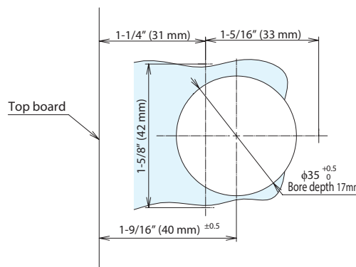
[Bore Dimensions]
