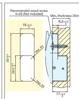
Bore Dimensions (For thickness 20~29 mm)
