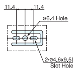
DETAIL L
