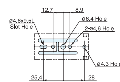
DETAIL K
