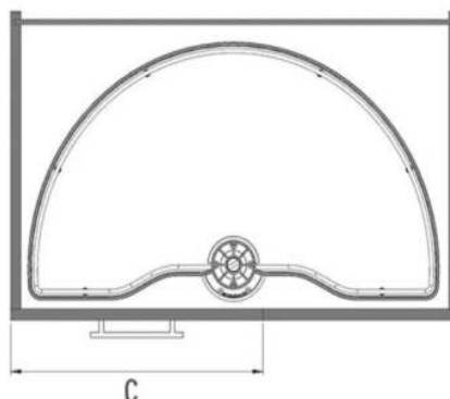
TURNING BASKET SET S-3012 W=420mm x D=650mm x
