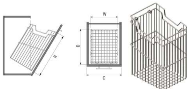
TILT OUT HAMPER UNIT
