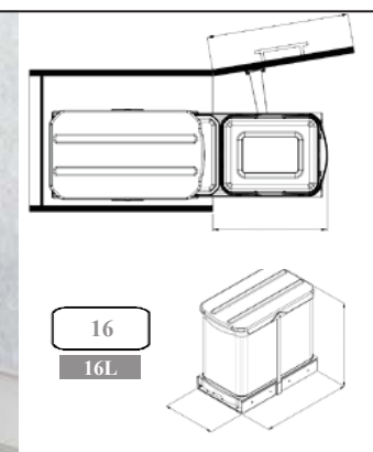
SINGLE PAIL WASTE BIN
