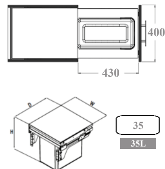
SINGLE PAIL WASTE BIN
